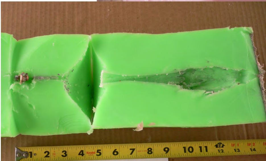
150 gr Nosler Ballistic Tip in 308 Win. The dark shading in the cavity is lead particles and lead dust.
