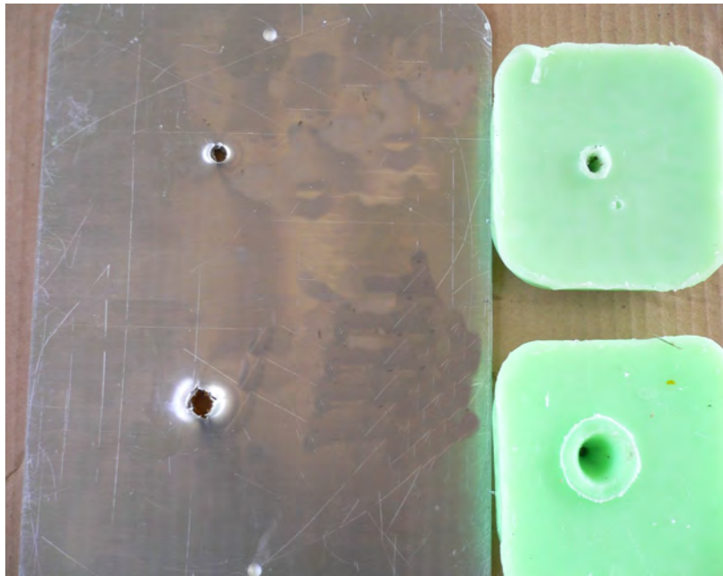
270 Winchester, 130 gr @ 1800 fps (reduced load) 1 1/2" media + 1/8" aluminum
